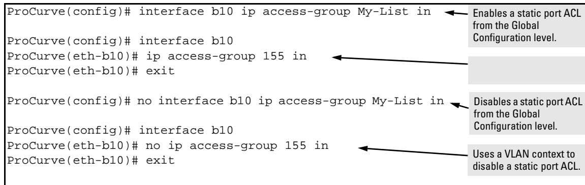
Figure 9-15. Methods for Enabling and Disabling ACLs
